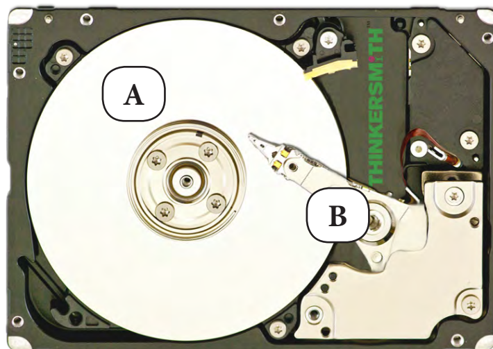
A) Spinning Storage Platter B) Read/Write Head
